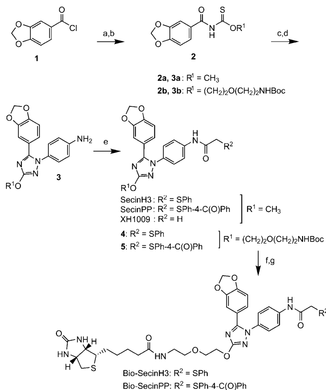
Scheme 1. Synthesis of the Secin derivatives used: a) KSCN, acetone, 60 °C; b) R'OH, acetone, 50 °C, 83 %; c) 4-nitrophenylhydrazine, EtOH, 80 °C, 70%; d) Fe/HCl, NH 4 Cl, MeOH/H 2 O, 65 °C, 64 %; e) R 2 CH 2 COOH, HBTU/NEt 3 , DMF, 22 °C, 57%; f) TFA/CH 2 Cl 2 , 94 %; g) D-(+)-biotin, HBTU/NEt 3 , DMF, 69%. Boc = tert -butoxycarbonyl, DMF = N,N-dimethylformamide, HBTU = O-benzotriazole-N,N,N',N'-tetramethyluronium hexafluorophosphate, TFA = trifluoroacetic acid.
