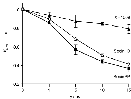
Figure 1. Inhibition by SecinH3, SecinPP, and XH1009 of guanine-nucleotide exchange on [\Delta 17]\text{Arf1} catalyzed by the Sec7 domain of cytohesin 2 (ARNO; tryptophan fluorescence assay). [10] c = inhibitor concentration, v_{\text{rel}} = relative initial rate.
