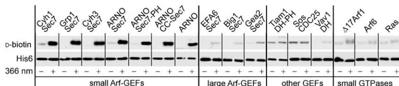
Figure 3. Photoaffinity labeling of GEF functional domains and small GTPases (2.5 \mu M) with Bio-SecinPP (2.5 \mu M). Irradiation: 100 mW, 1 min.
