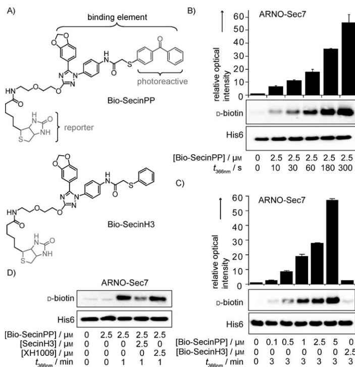
Figure 2. A) Structures of Bio-SecinPP and Bio-SecinH3. B),C) Photoaffinity labeling of ARNO-Sec7 with Bio-SecinPP with increasing irradiation time (B) and increasing concentration (C). D) Competition experiment with an equal amount of SecinH3 or XH1009.
